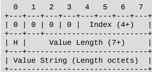
Figure 8: Literal Header Field without Indexing — Indexed Name
