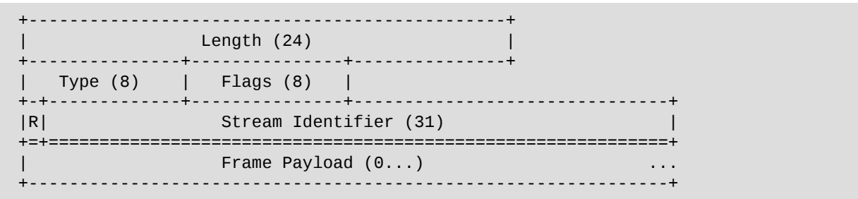
Figure 1: Frame Layout
