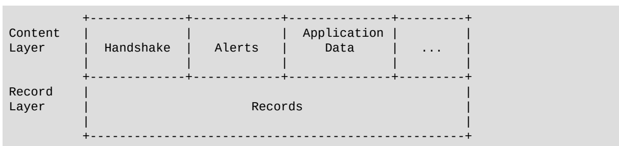
Figure 1: TLS Layers
